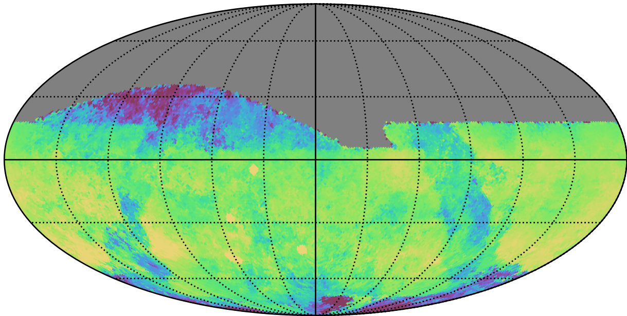
baseline_v2.0_10yrs All sky i band: Median skyBrightness
