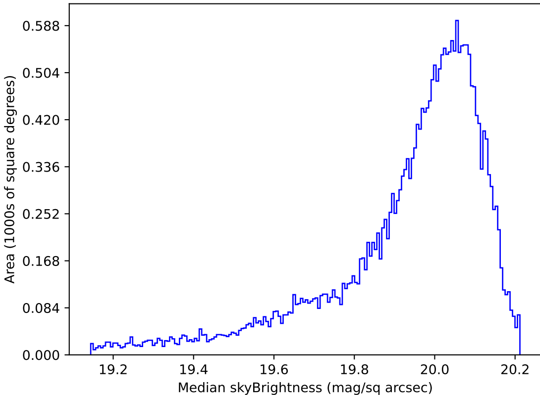
baseline_v2.0_10yrs All sky i band: Median skyBrightness
