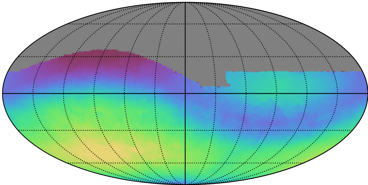
baseline_v2.0_10yrs All sky g band: Median skyBrightness
