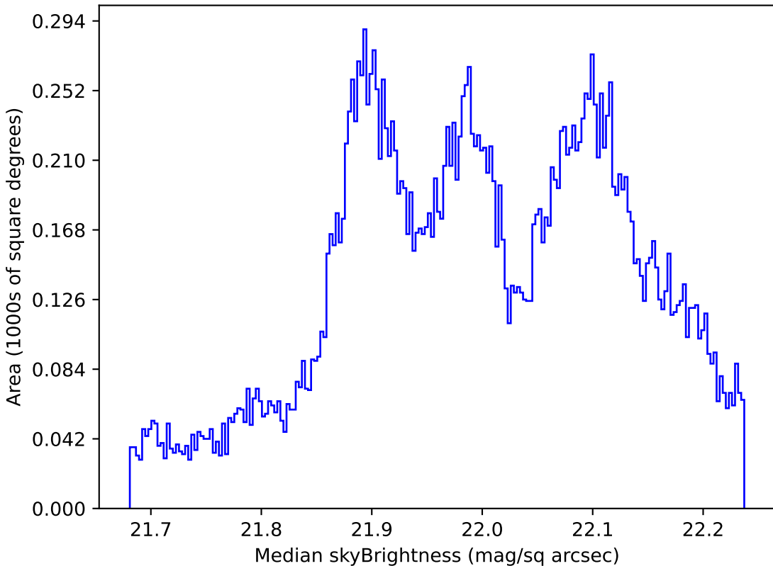
baseline_v2.0_10yrs All sky g band: Median skyBrightness
