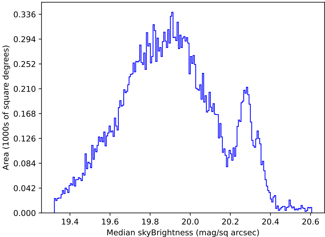
baseline_v2.0_10yrs All sky all bands: Median skyBrightness
