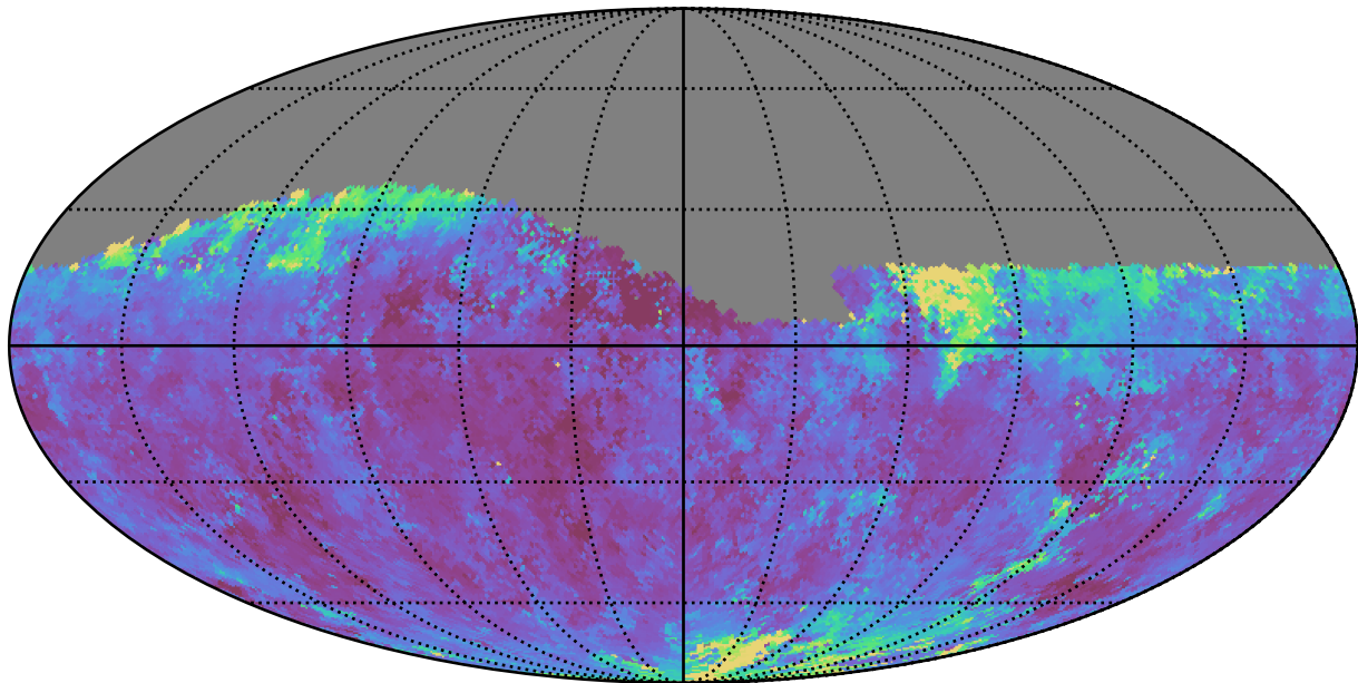
baseline_v2.0_10yrs Yr 1 z band: Median seeingGeom
