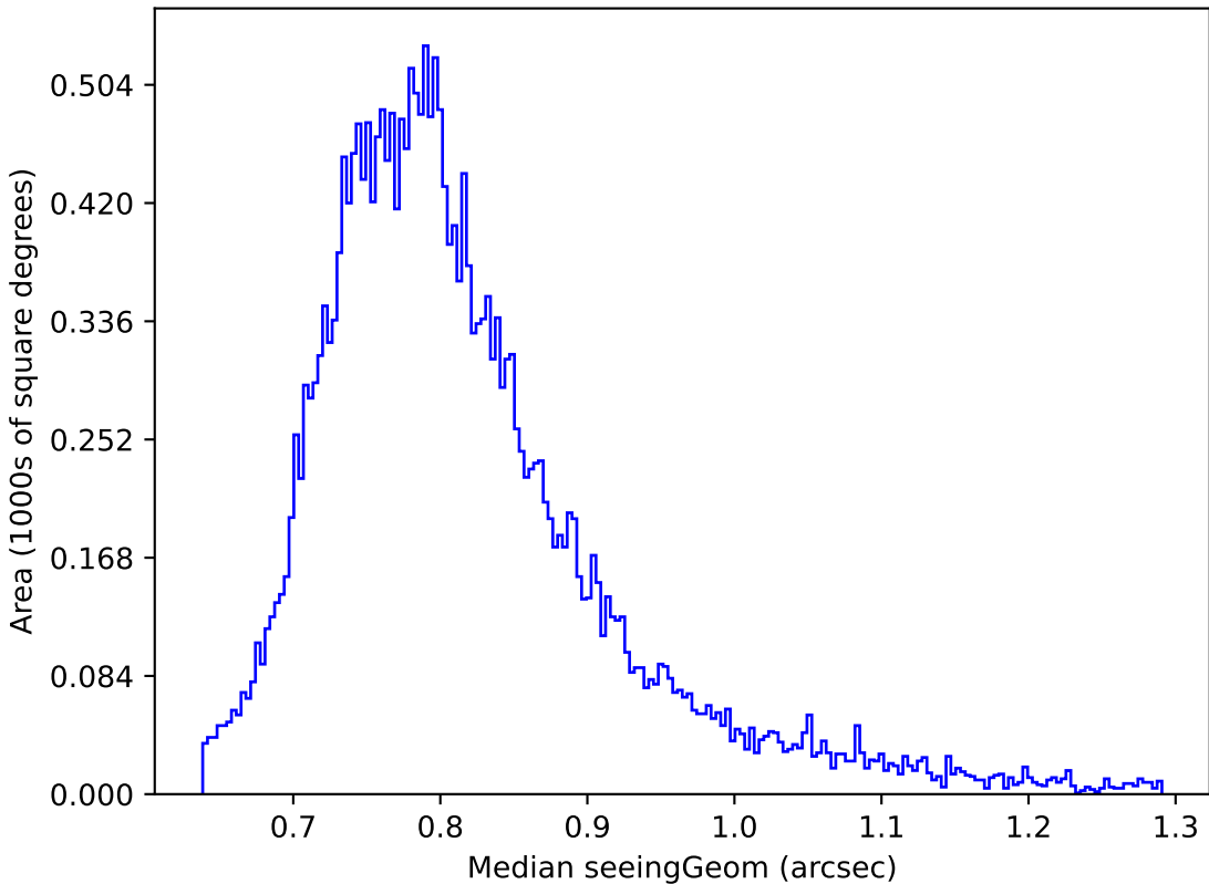
baseline_v2.0_10yrs Yr 1 z band: Median seeingGeom
