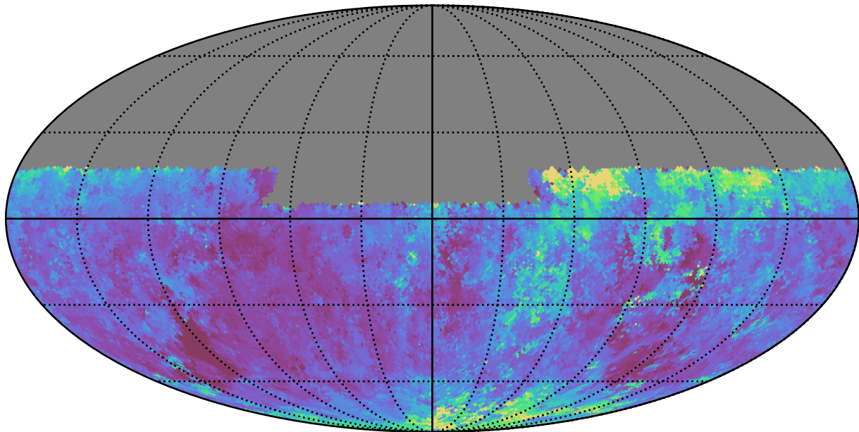
baseline_v2.0_10yrs Yr 1 y band: Median seeingGeom
