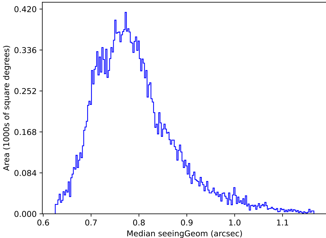
baseline_v2.0_10yrs Yr 1 y band: Median seeingGeom
