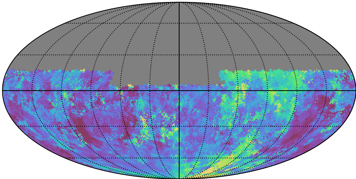
baseline_v2.0_10yrs Yr 1 u band: Median seeingGeom
