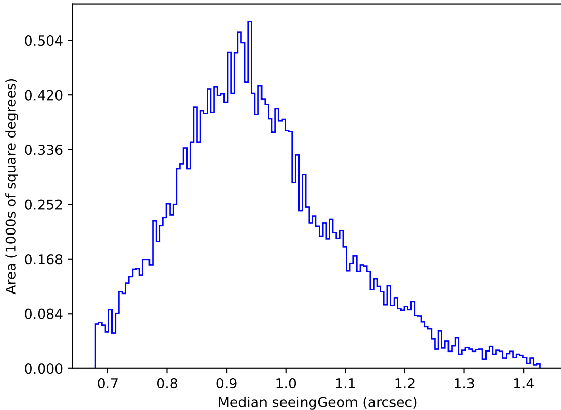
baseline_v2.0_10yrs Yr 1 u band: Median seeingGeom
