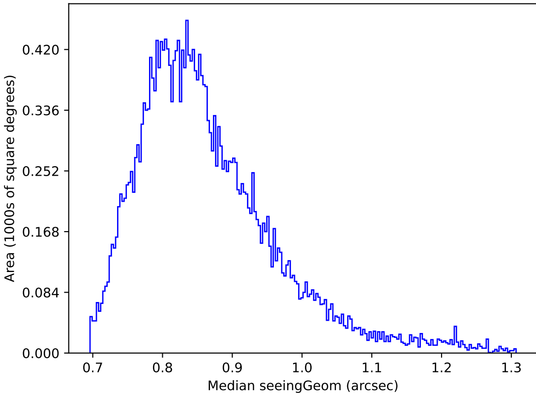
baseline_v2.0_10yrs Yr 1 r band: Median seeingGeom
