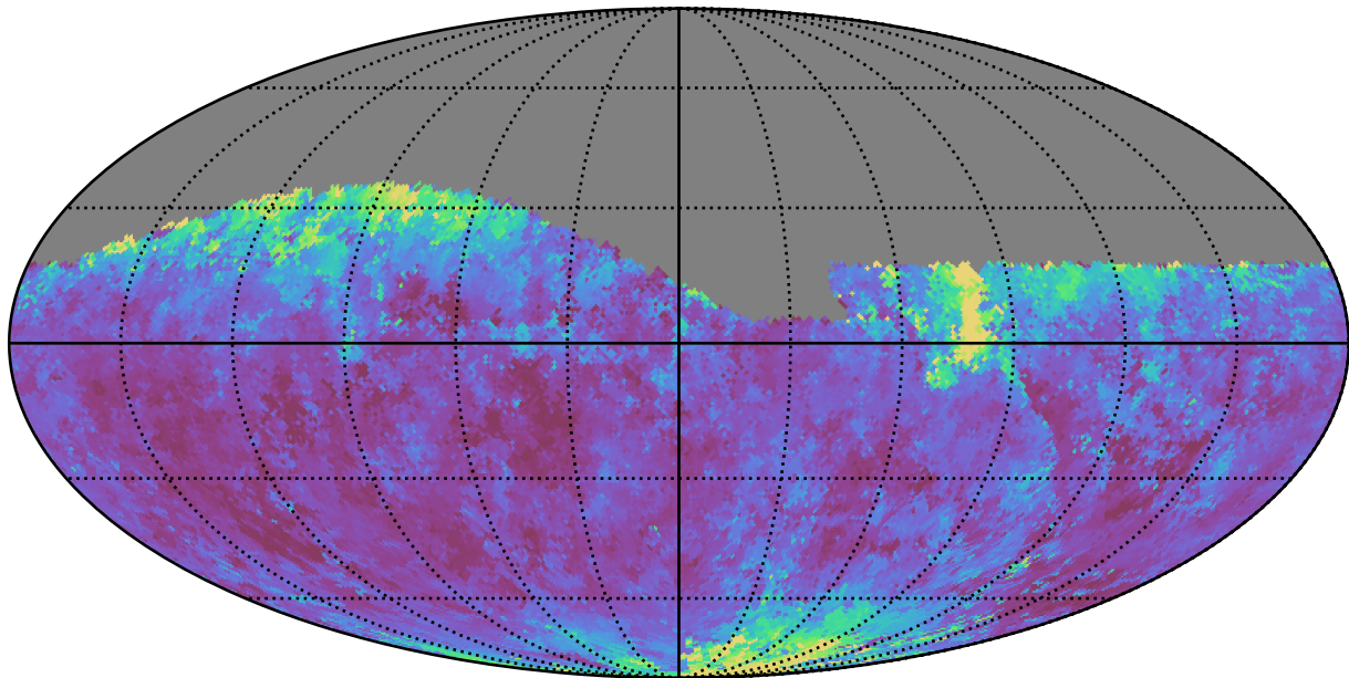
baseline_v2.0_10yrs Yr 1 i band: Median seeingGeom
