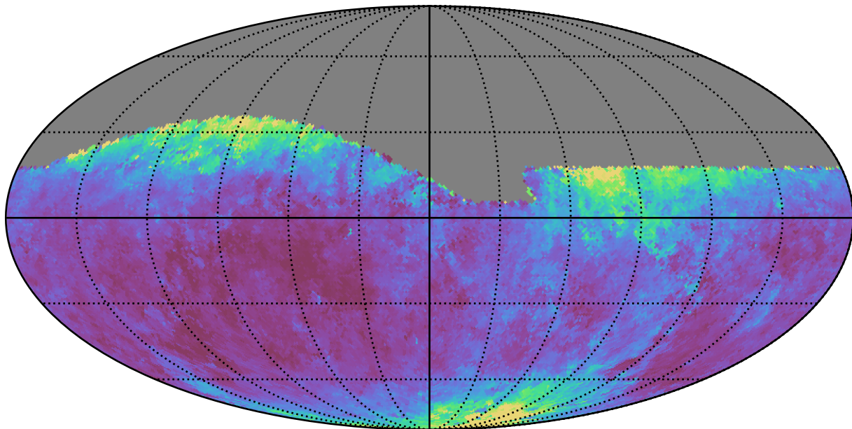
baseline_v2.0_10yrs Yr 1 all bands: Median seeingGeom
