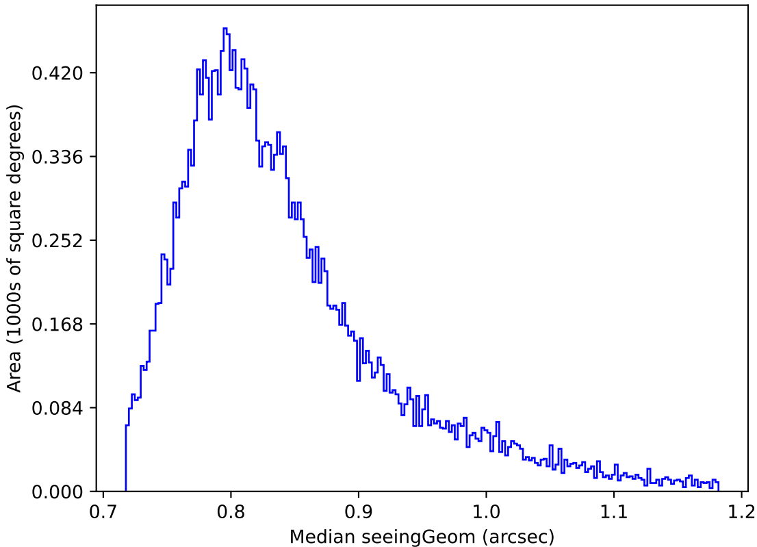
baseline_v2.0_10yrs Yr 1 all bands: Median seeingGeom
