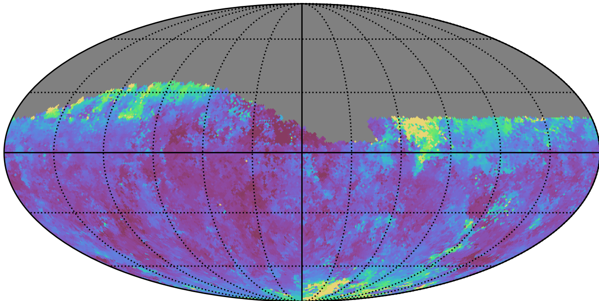
baseline_v2.0_10yrs Yr 1 z band: Median seeingEff
