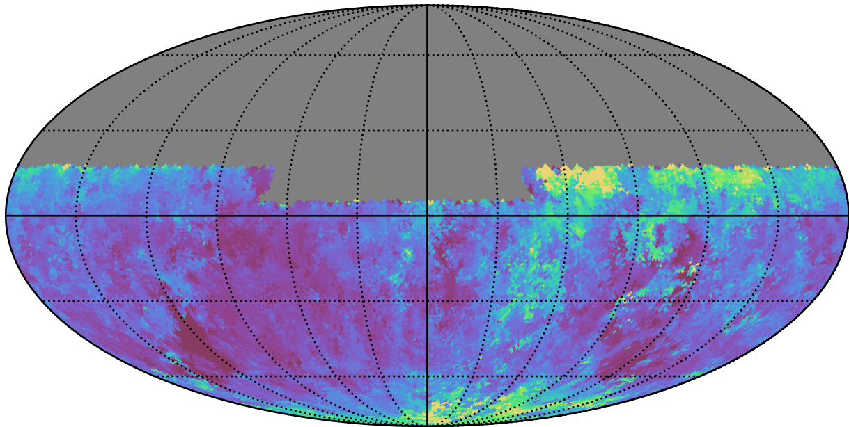
baseline_v2.0_10yrs Yr 1 y band: Median seeingEff
