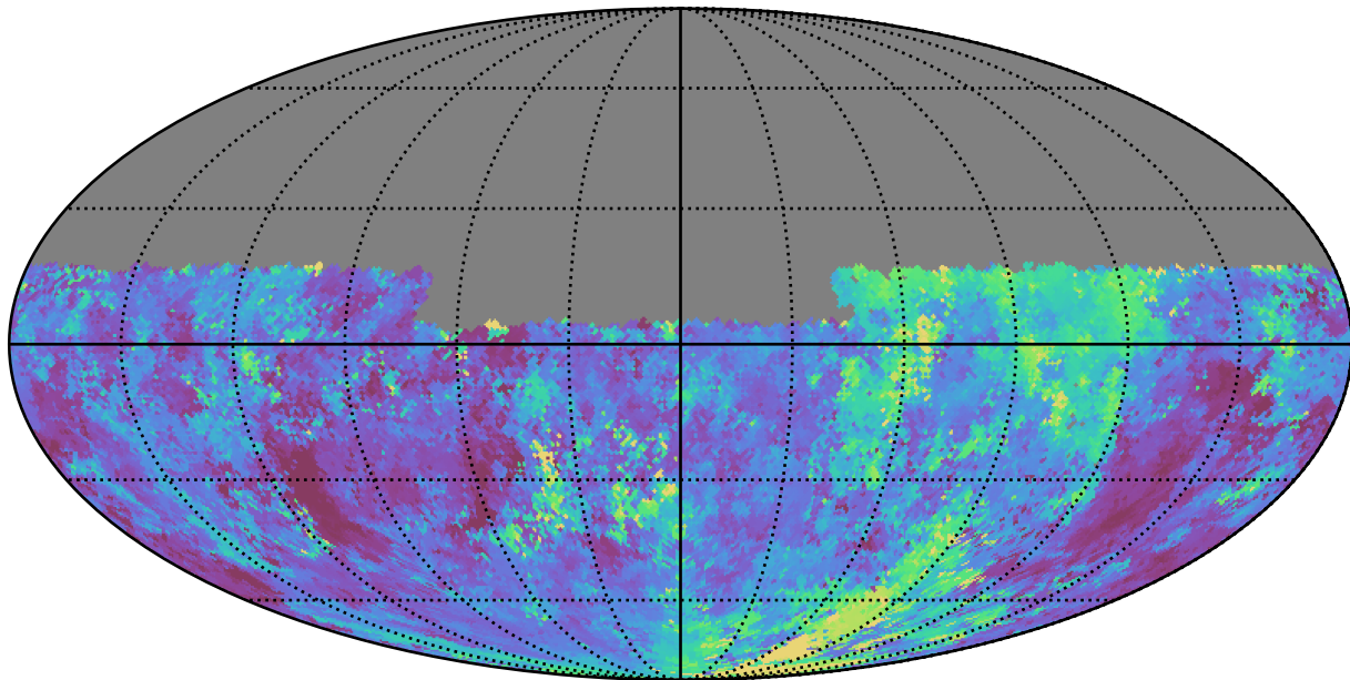
baseline_v2.0_10yrs Yr 1 u band: Median seeingEff
