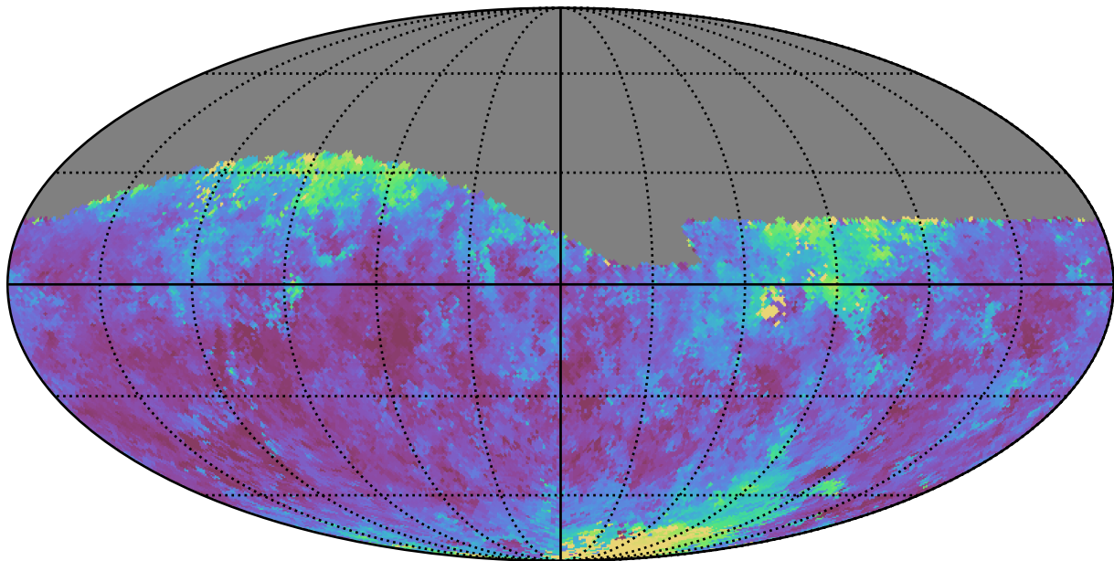
baseline_v2.0_10yrs Yr 1 r band: Median seeingEff
