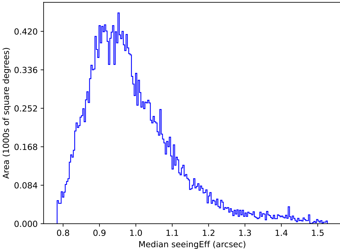
baseline_v2.0_10yrs Yr 1 r band: Median seeingEff
