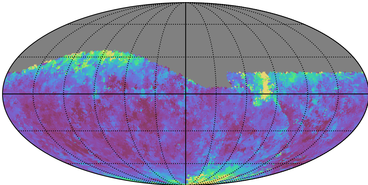
baseline_v2.0_10yrs Yr 1 i band: Median seeingEff
