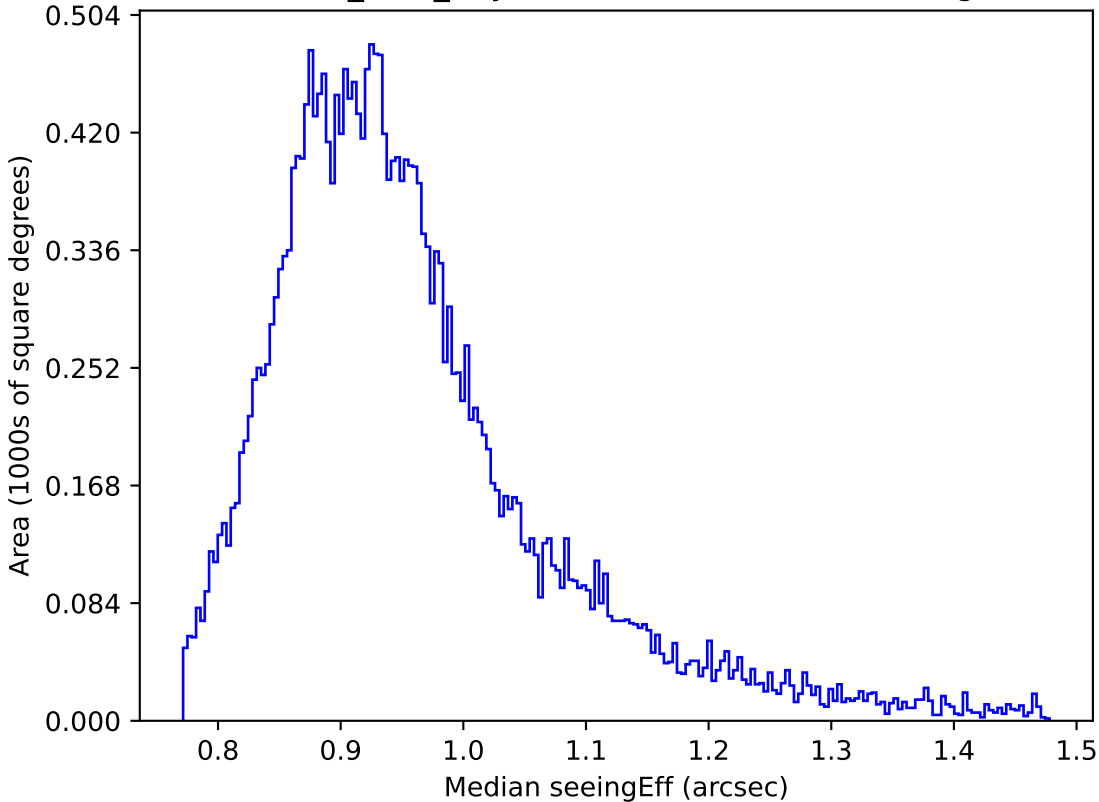
baseline_v2.0_10yrs Yr 1 i band: Median seeingEff
