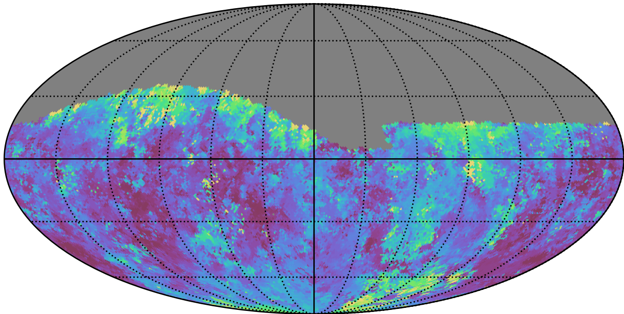
baseline_v2.0_10yrs Yr 1 g band: Median seeingEff
