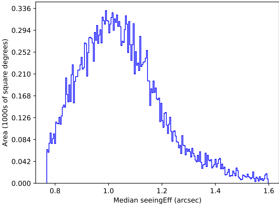
baseline_v2.0_10yrs Yr 1 g band: Median seeingEff
