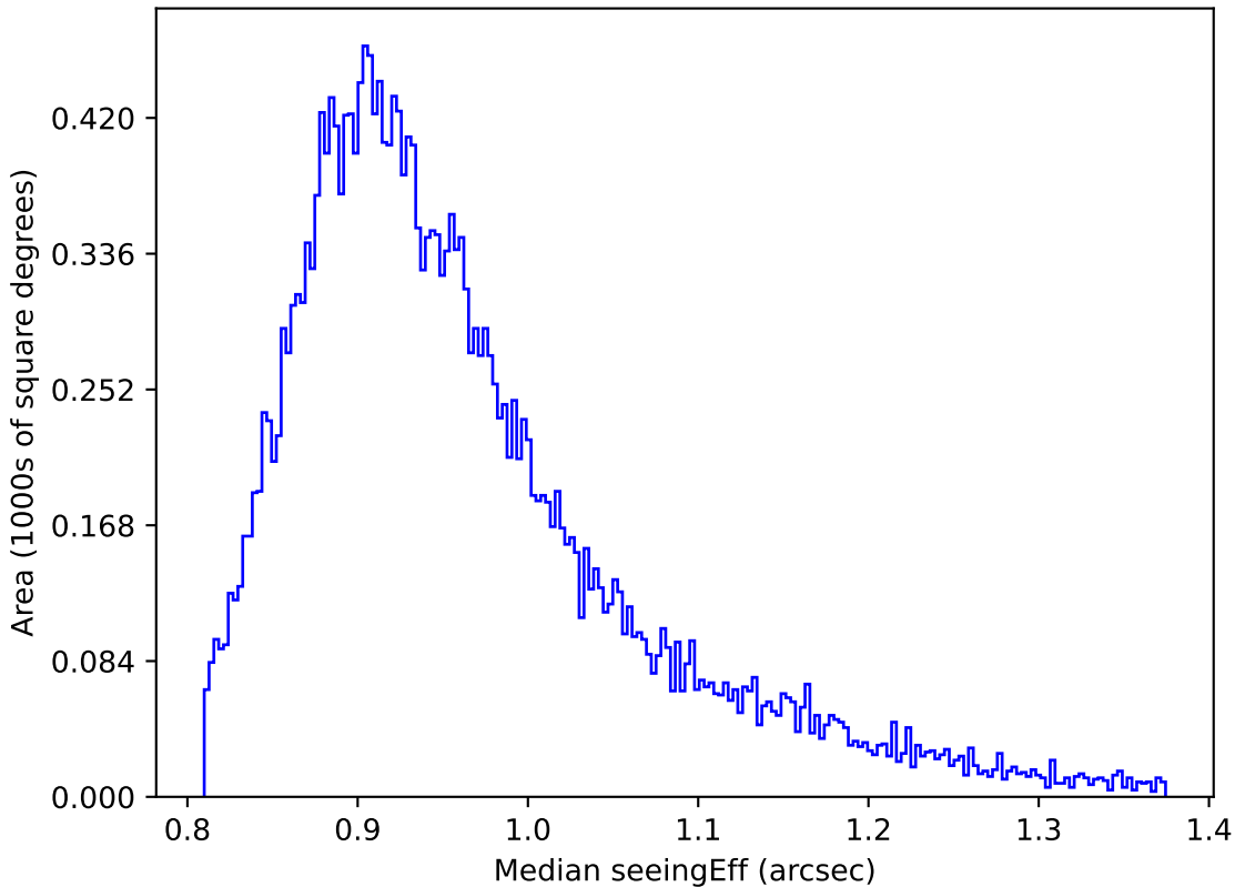
baseline_v2.0_10yrs Yr 1 all bands: Median seeingEff
