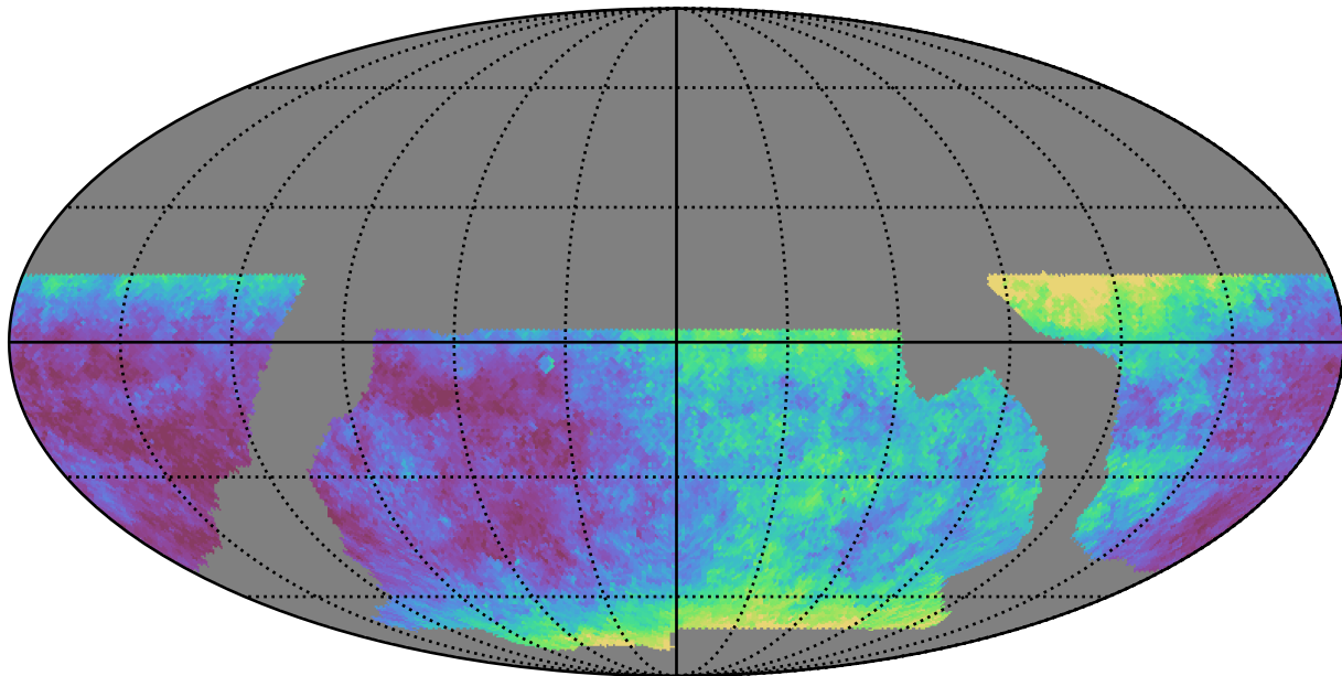
baseline_v2.0_10yrs WFD z band: Median seeingEff
