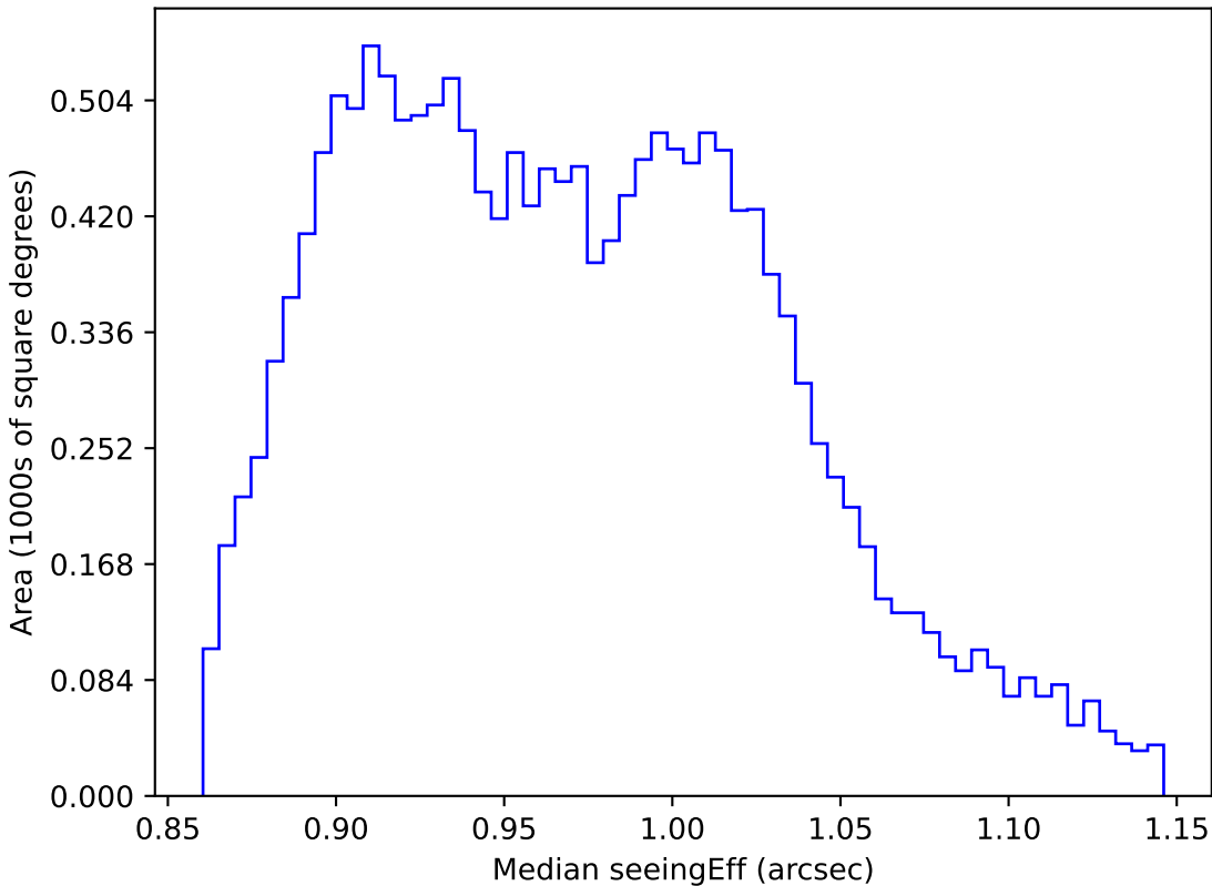
baseline_v2.0_10yrs WFD z band: Median seeingEff
