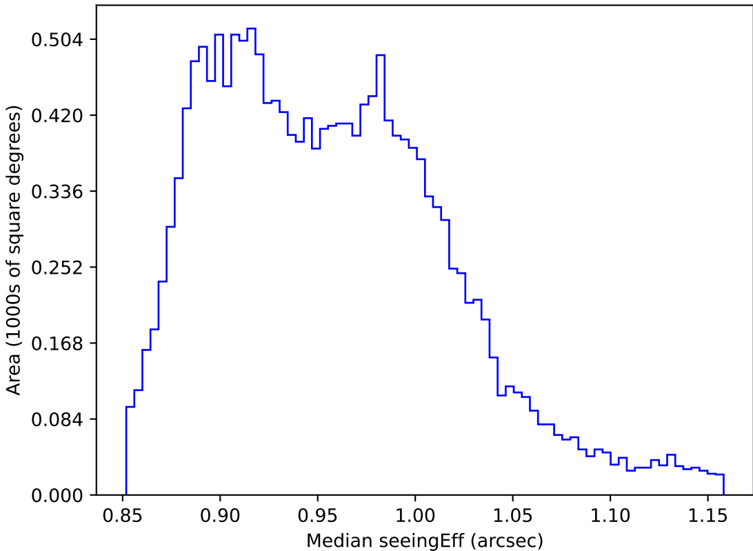
baseline_v2.0_10yrs WFD y band: Median seeingEff
