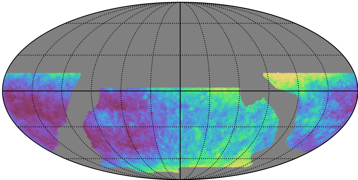
baseline_v2.0_10yrs WFD r band: Median seeingEff
