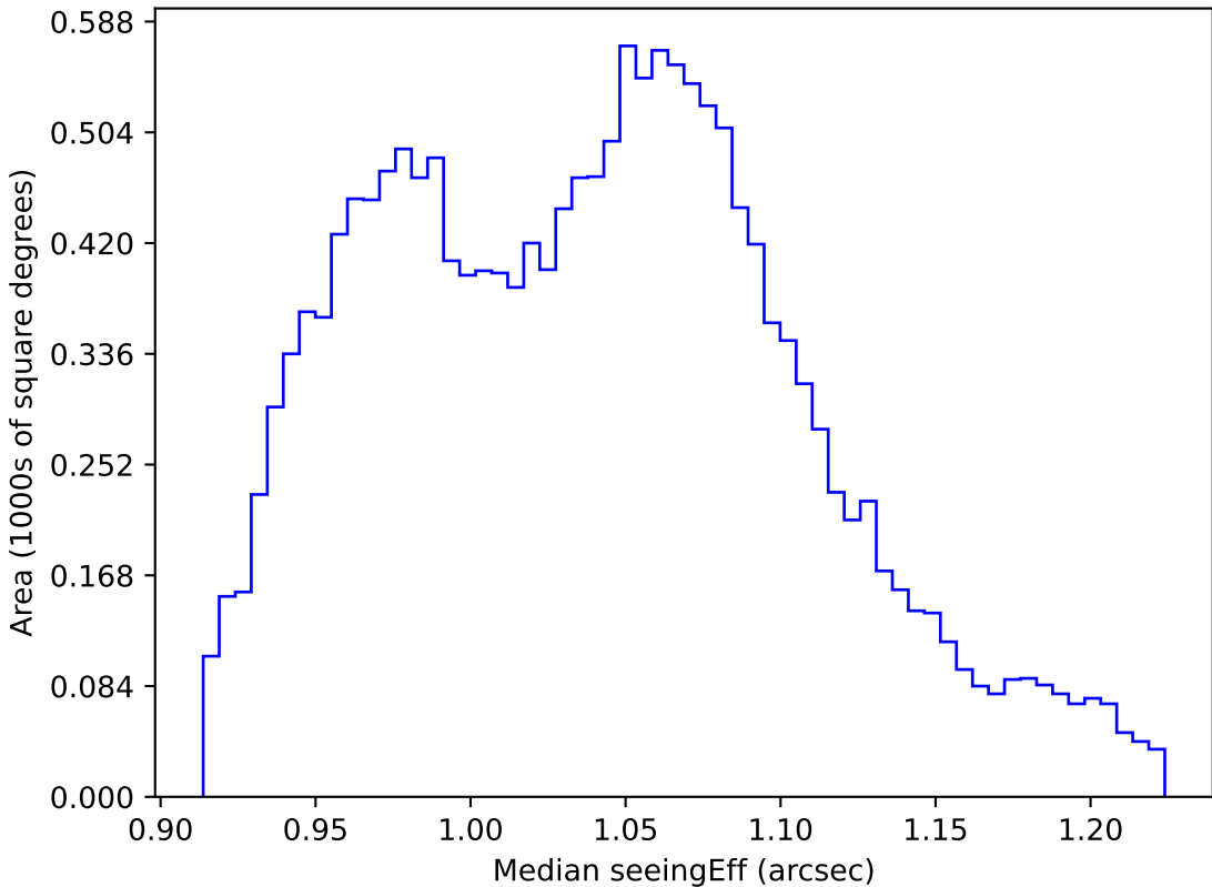
baseline_v2.0_10yrs WFD r band: Median seeingEff
