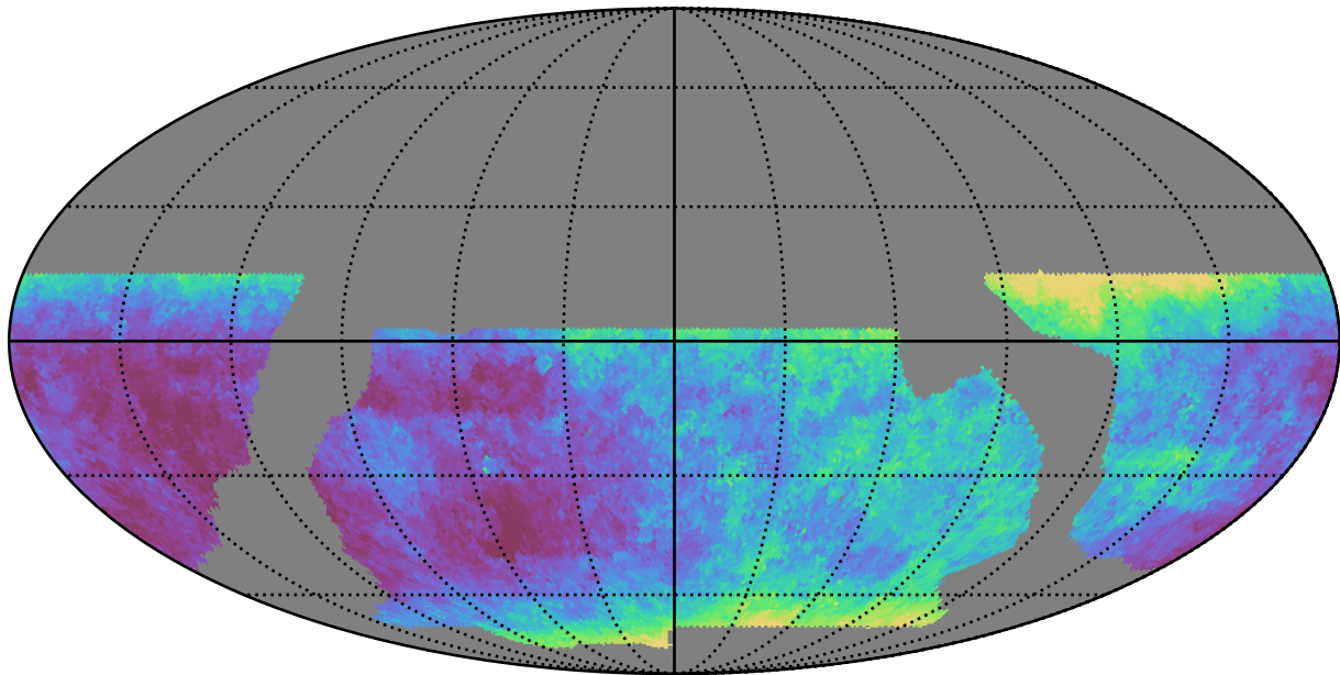
baseline_v2.0_10yrs WFD i band: Median seeingEff
