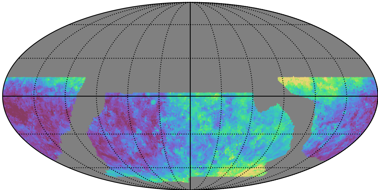
baseline_v2.0_10yrs WFD g band: Median seeingEff
