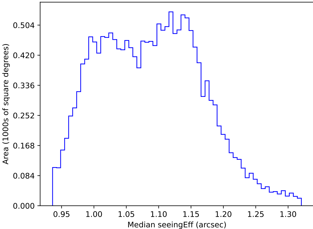
baseline_v2.0_10yrs WFD g band: Median seeingEff
