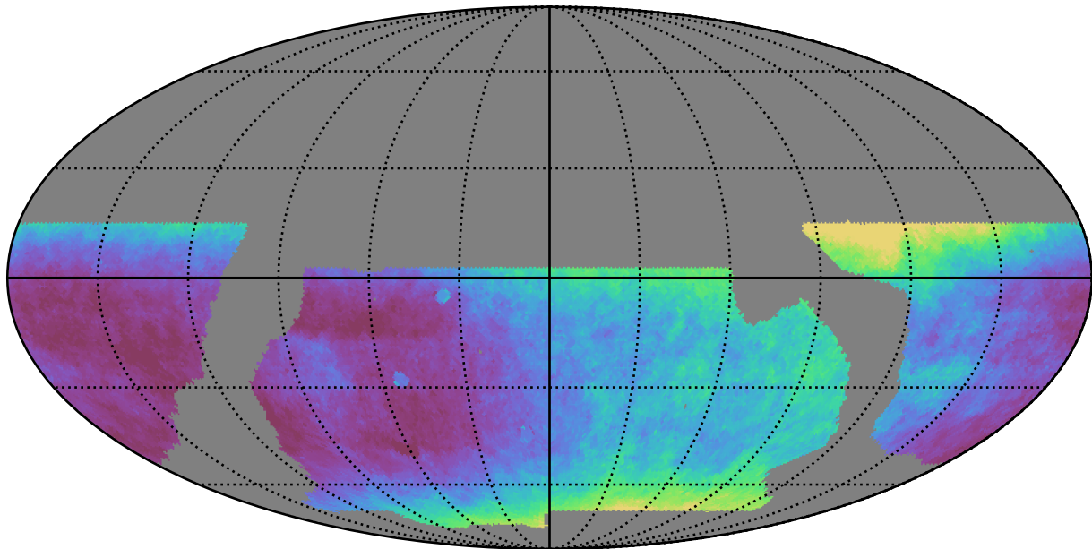
baseline_v2.0_10yrs WFD all bands: Median seeingEff
