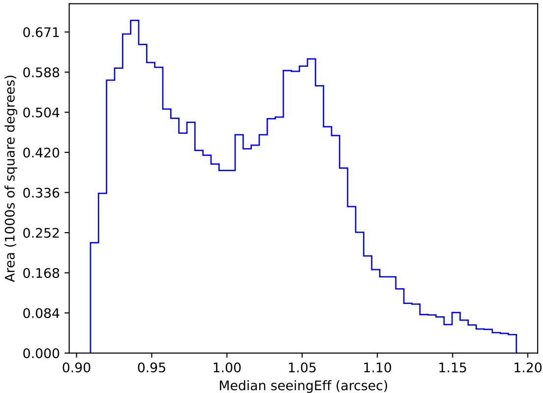
baseline_v2.0_10yrs WFD all bands: Median seeingEff
