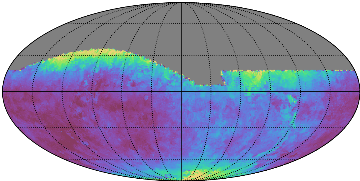
baseline_v2.0_10yrs All sky z band: Median seeingEff
