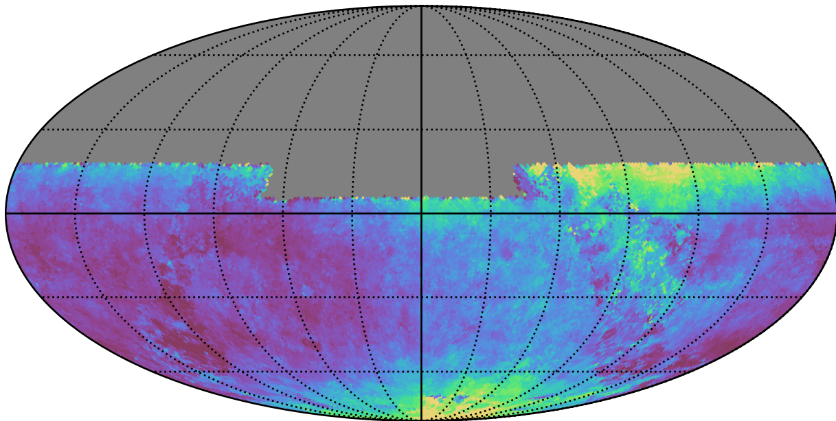
baseline_v2.0_10yrs All sky y band: Median seeingEff
