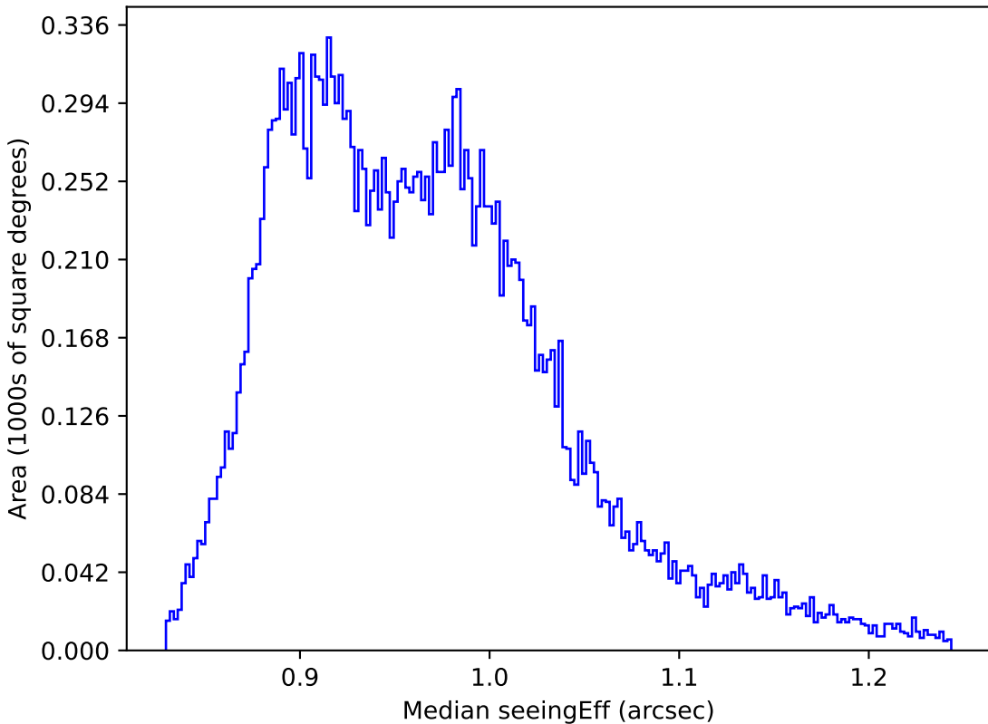
baseline_v2.0_10yrs All sky y band: Median seeingEff
