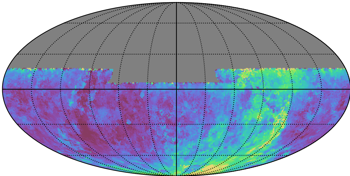
baseline_v2.0_10yrs All sky u band: Median seeingEff
