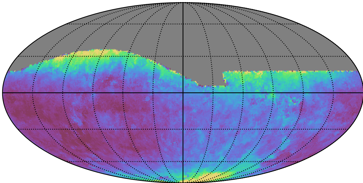
baseline_v2.0_10yrs All sky r band: Median seeingEff
