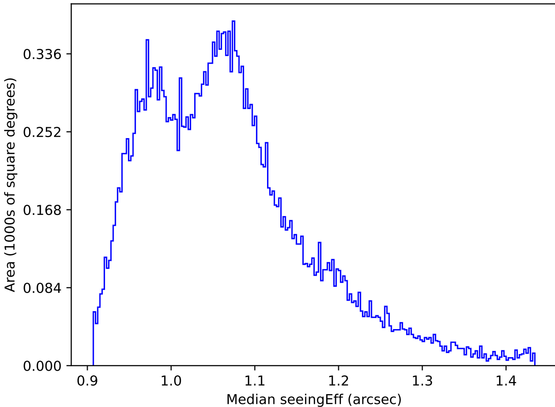
baseline_v2.0_10yrs All sky r band: Median seeingEff
