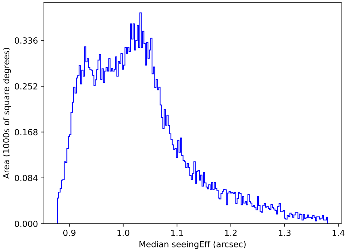
baseline_v2.0_10yrs All sky i band: Median seeingEff
