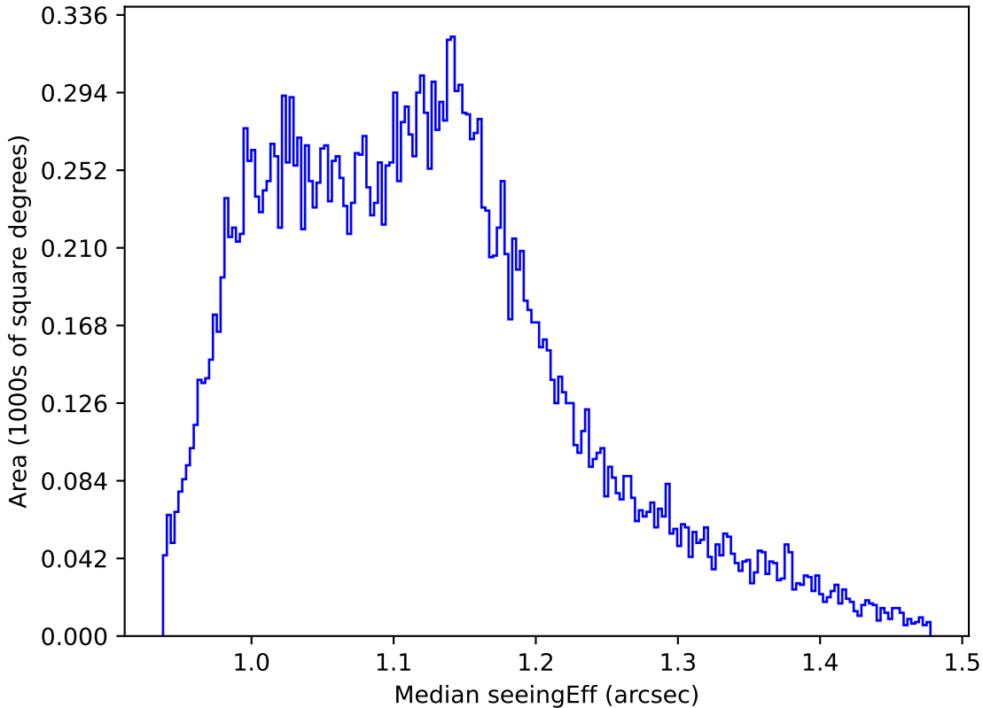
baseline_v2.0_10yrs All sky g band: Median seeingEff
