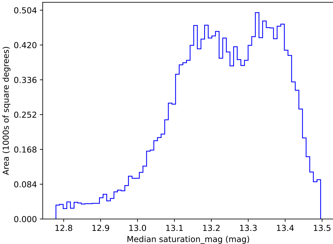
baseline_v2.0_10yrs WFD y band: Median saturation_mag
