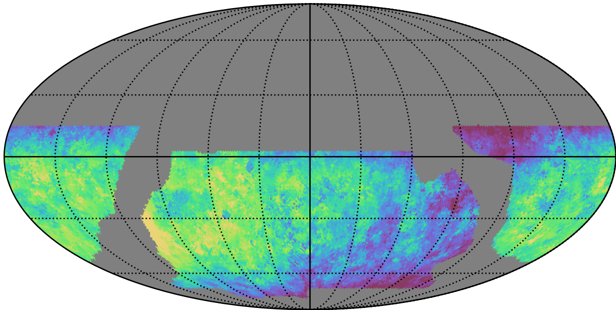
baseline_v2.0_10yrs WFD u band: Median saturation_mag
