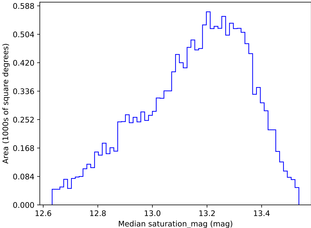
baseline_v2.0_10yrs WFD u band: Median saturation_mag
