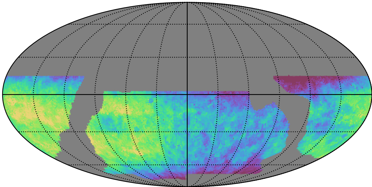
baseline_v2.0_10yrs WFD r band: Median saturation_mag
