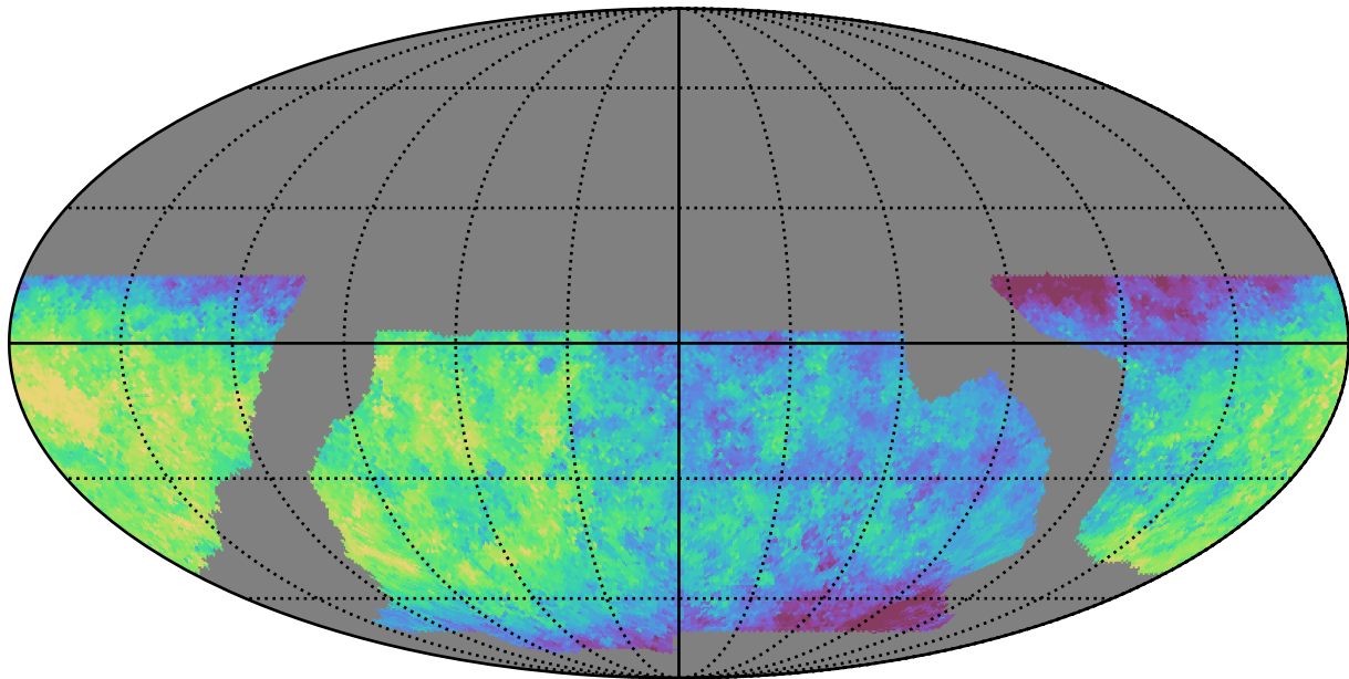
baseline_v2.0_10yrs WFD g band: Median saturation_mag
