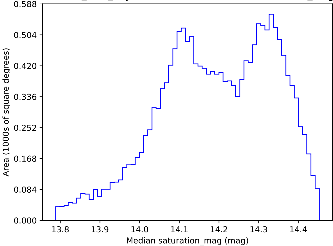
baseline_v2.0_10yrs WFD all bands: Median saturation_mag
