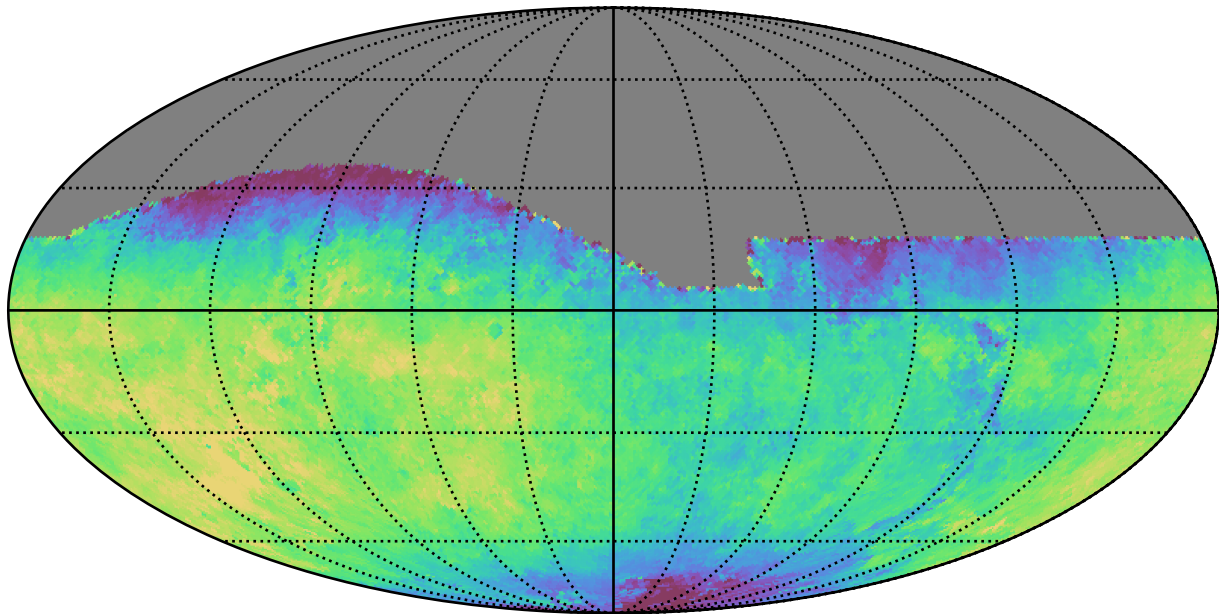
baseline_v2.0_10yrs All sky z band: Median saturation_mag
